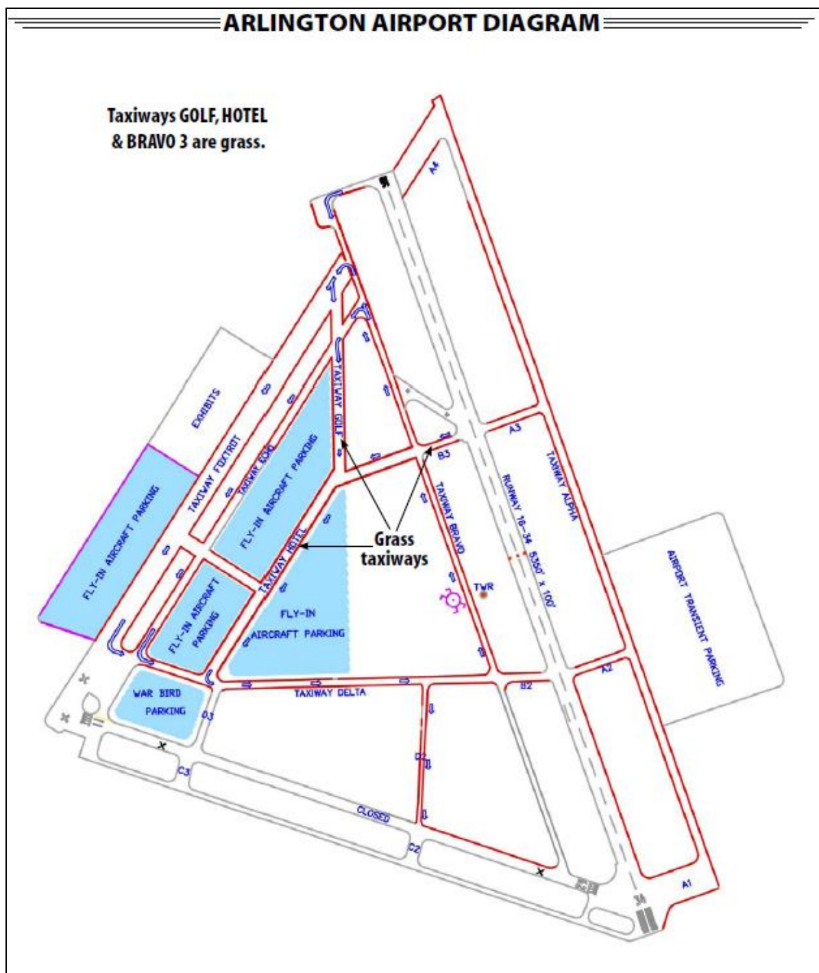
Arlington Airport Diagram and Parking Map
